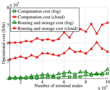
Fig. 10: Operational cost per year
