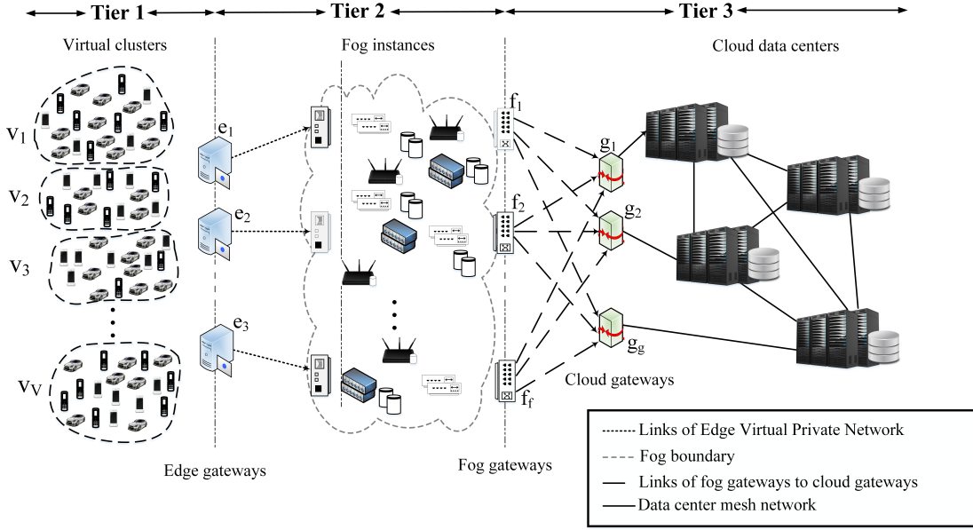
Fig. 2: Networking links and components of fog computing
