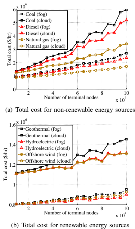
Fig. 12: Analysis of cost for renewable energy sources
