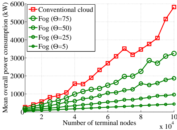
Fig. 6: Overall power consumption vs No. of TNs
